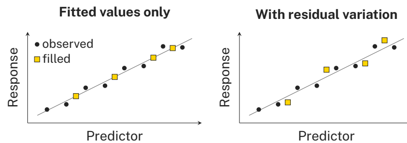
Figure 5. Fitted-value substitution and one illustrative stochastic alternative
